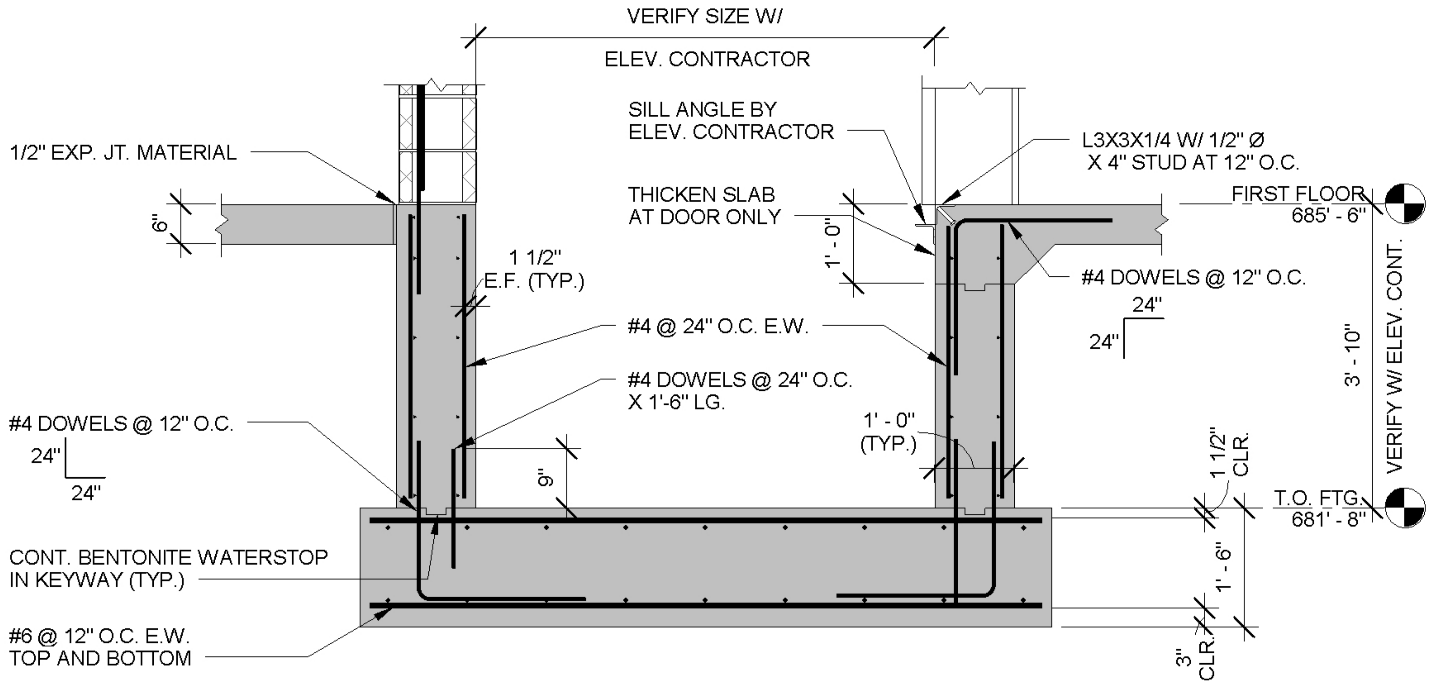
6 ELEVATOR FOUNDATION DETAIL SCALE: 1/2" = 1'-0"
