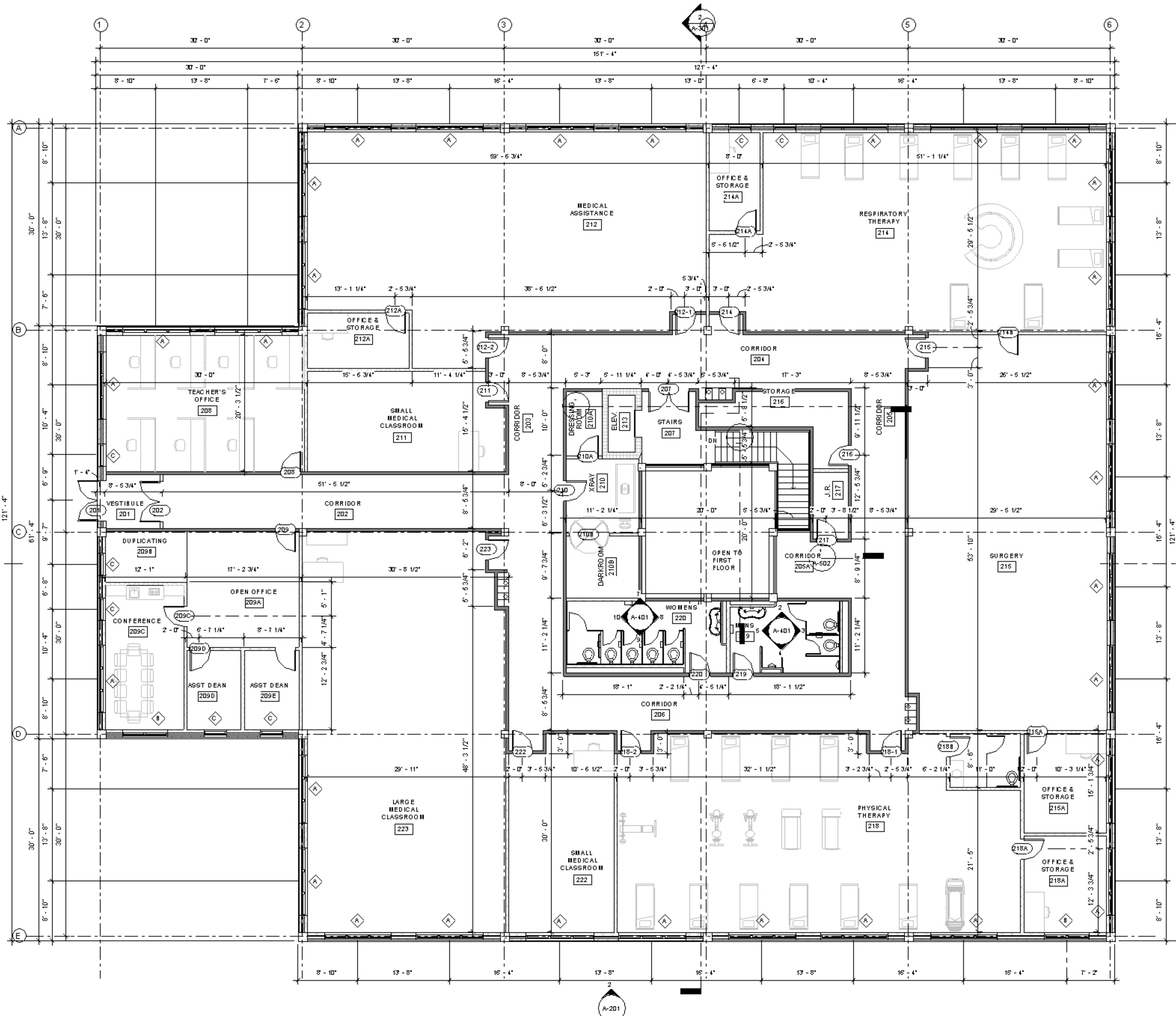
1 SECOND FLOOR PRESENTATION SCALE: 1/8" = 1'-0"
